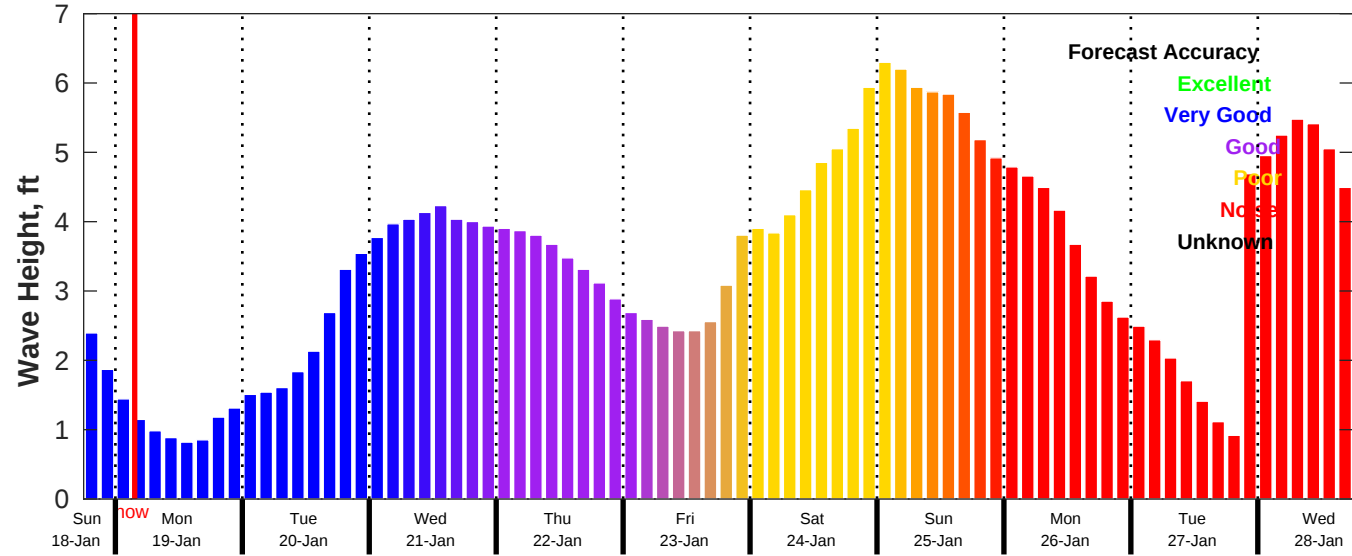
CMEMS Wave Forecast for NDBC 42019 from 18-Jan-2026 18:00:00 to 28-Jan-2026 18:00:00
