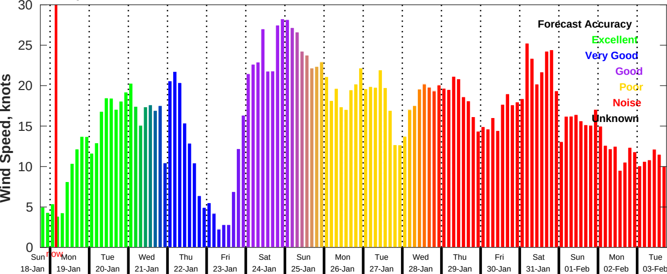
GFS Wind Speed Forecast for NDBC 42019 from 18-Jan-2026 18:00:00 to 03-Feb-2026 18:00:00
