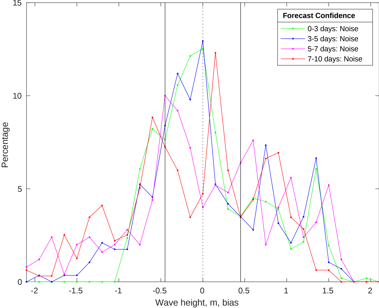
NDBC 42020 vs CMEMS Waves Bias Histogram: 19-Jan-2026
