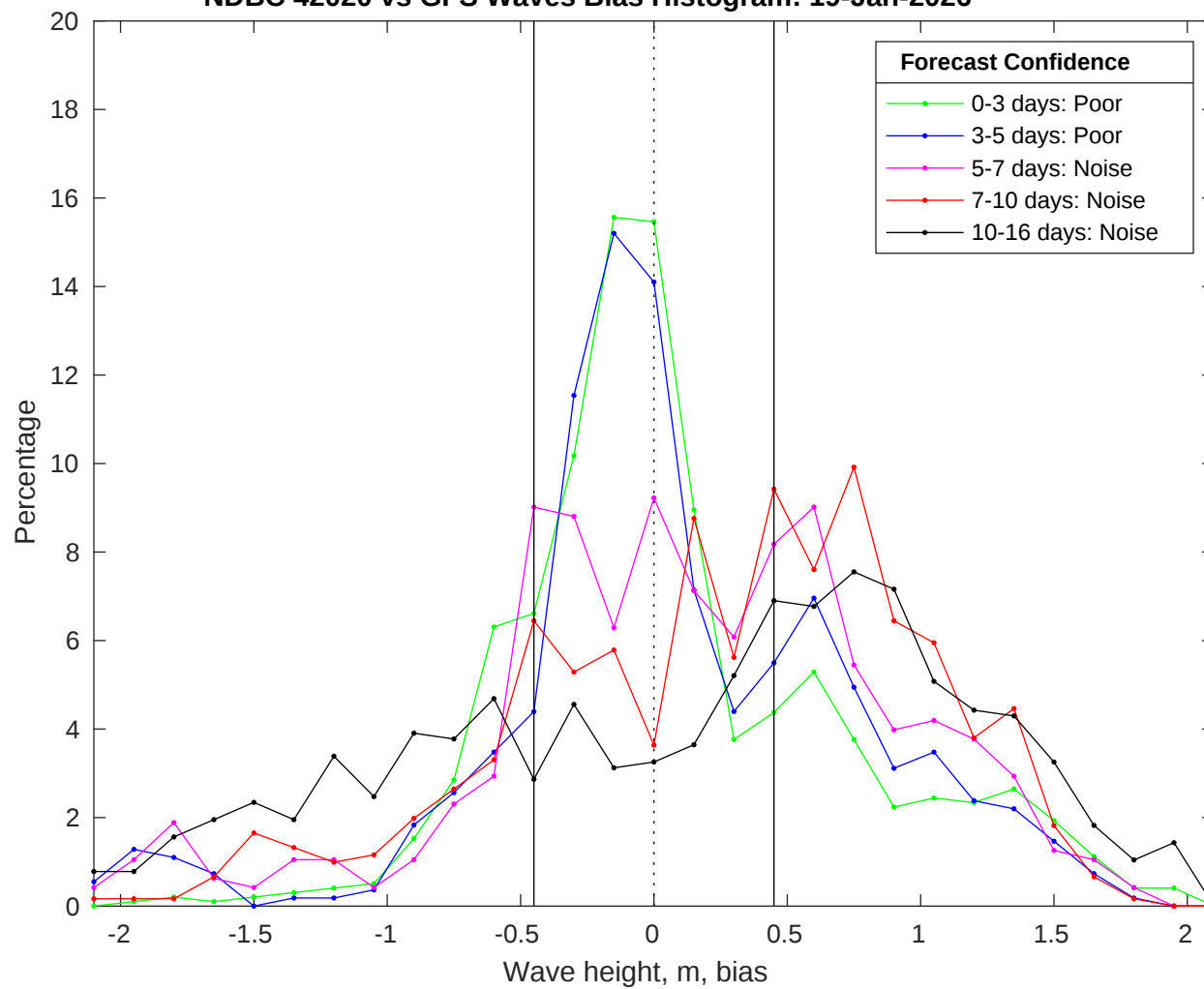
NDBC 42020 vs GFS Waves Bias Histogram: 19-Jan-2026
