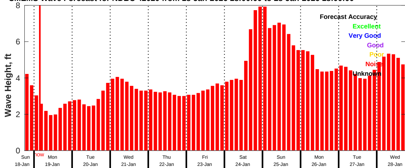
CMEMS Wave Forecast for NDBC 42020 from 18-Jan-2026 18:00:00 to 28-Jan-2026 18:00:00
