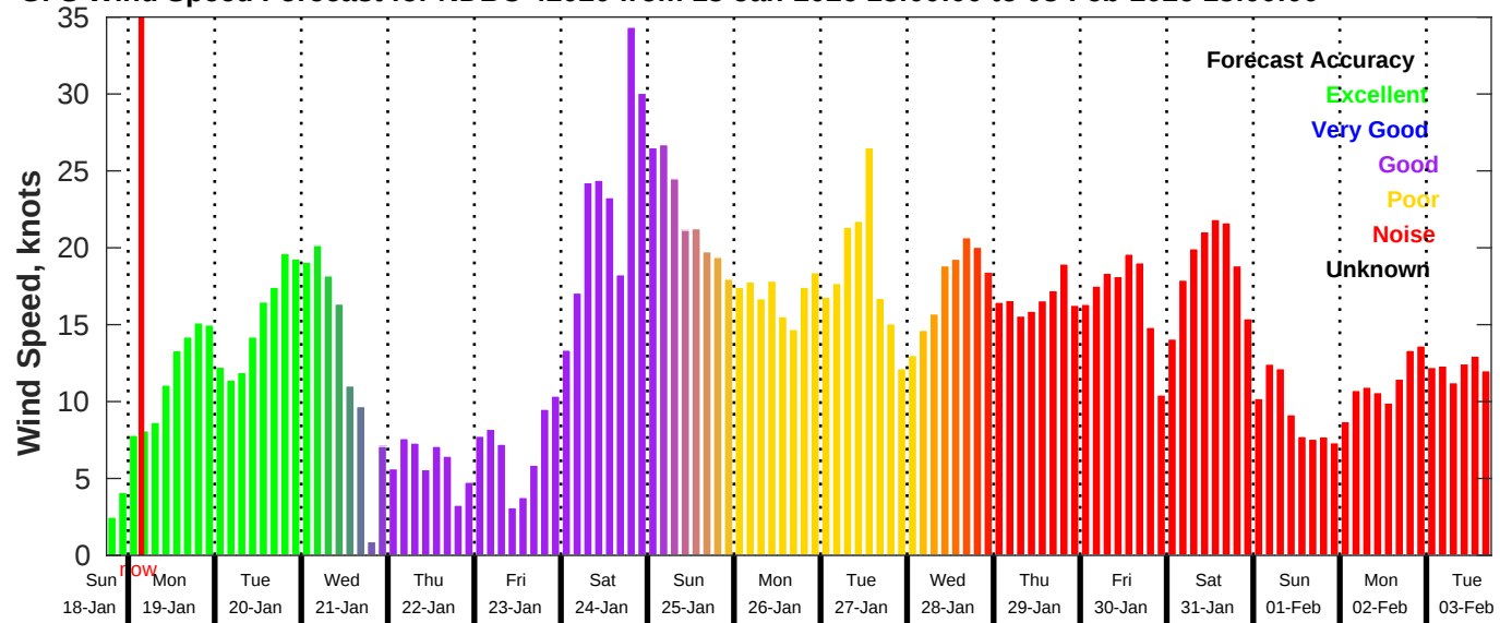
GFS Wind Speed Forecast for NDBC 42020 from 18-Jan-2026 18:00:00 to 03-Feb-2026 18:00:00
