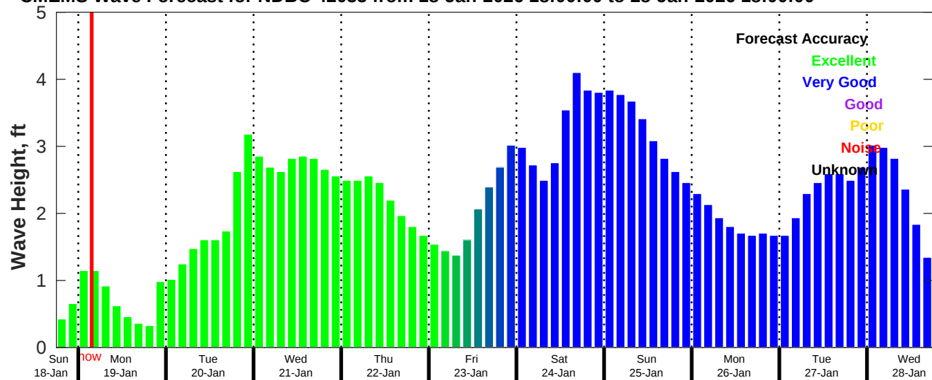
CMEMS Wave Forecast for NDBC 42035 from 18-Jan-2026 18:00:00 to 28-Jan-2026 18:00:00
