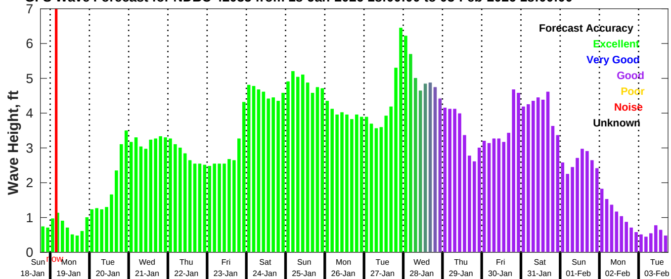
GFS Wave Forecast for NDBC 42035 from 18-Jan-2026 18:00:00 to 03-Feb-2026 18:00:00
