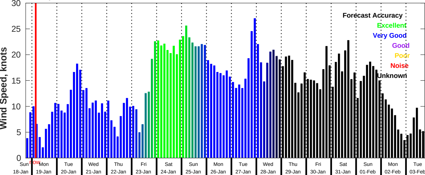
GFS Wind Speed Forecast for NDBC 42035 from 18-Jan-2026 18:00:00 to 03-Feb-2026 18:00:00
