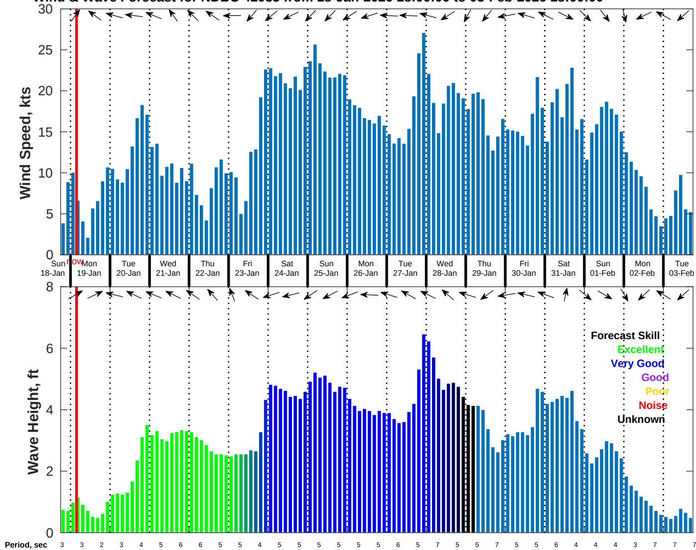
Wind & Wave Forecast for NDBC 42035 from 18-Jan-2026 18:00:00 to 03-Feb-2026 18:00:00
