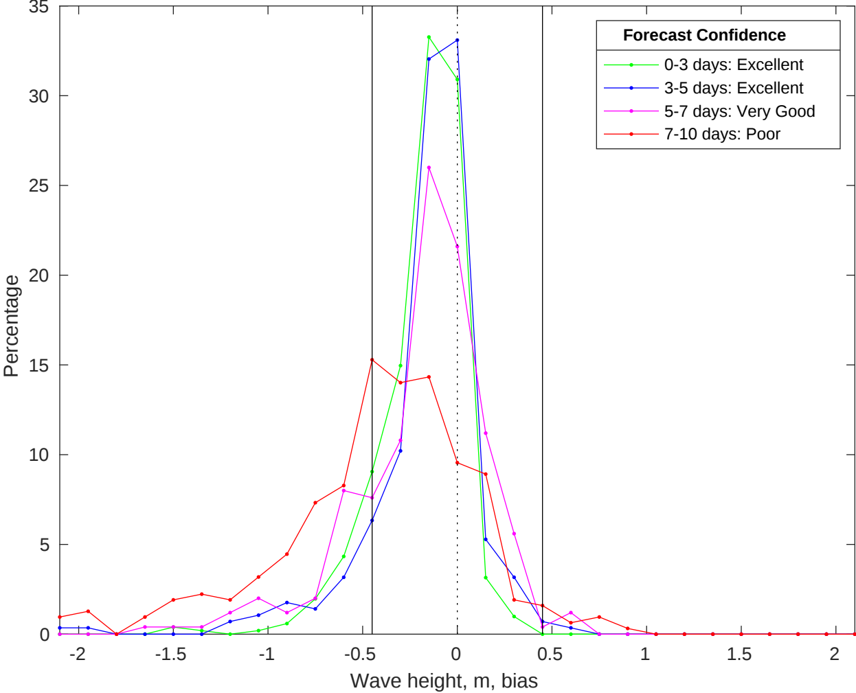
NDBC 42036 vs CMEMS Waves Bias Histogram: 19-Jan-2026
