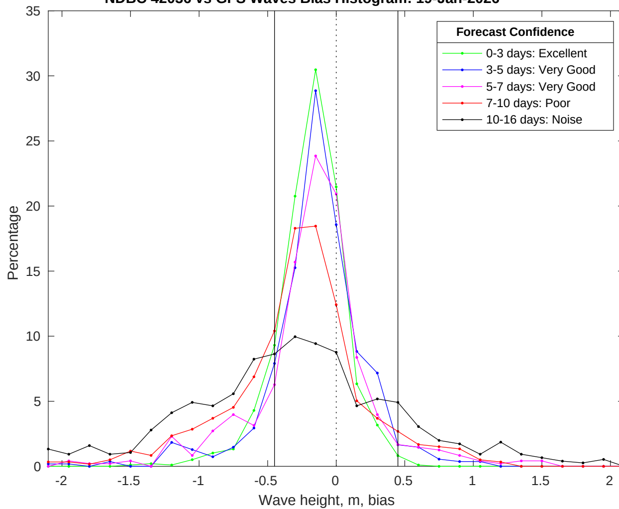
NDBC 42036 vs GFS Waves Bias Histogram: 19-Jan-2026
