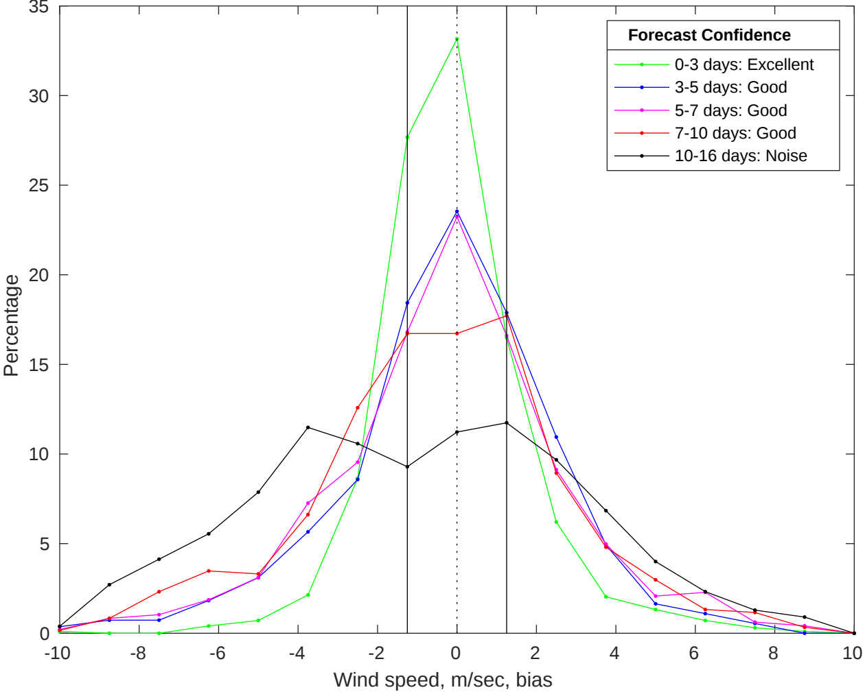
NDBC 42036 vs GFS Winds Bias Histogram: 19-Jan-2026
