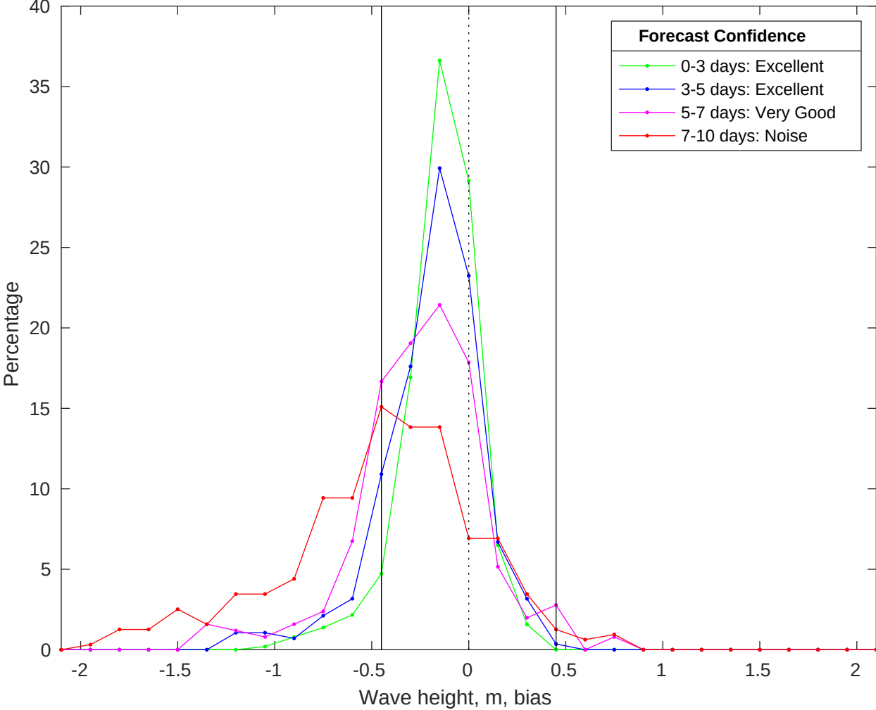
NDBC 42040 vs CMEMS Waves Bias Histogram: 19-Jan-2026
