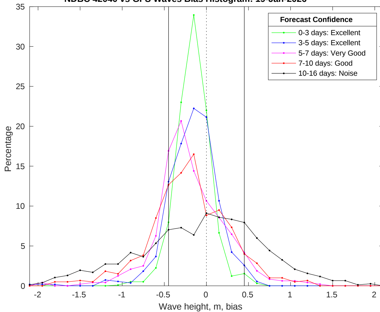
NDBC 42040 vs GFS Waves Bias Histogram: 19-Jan-2026
