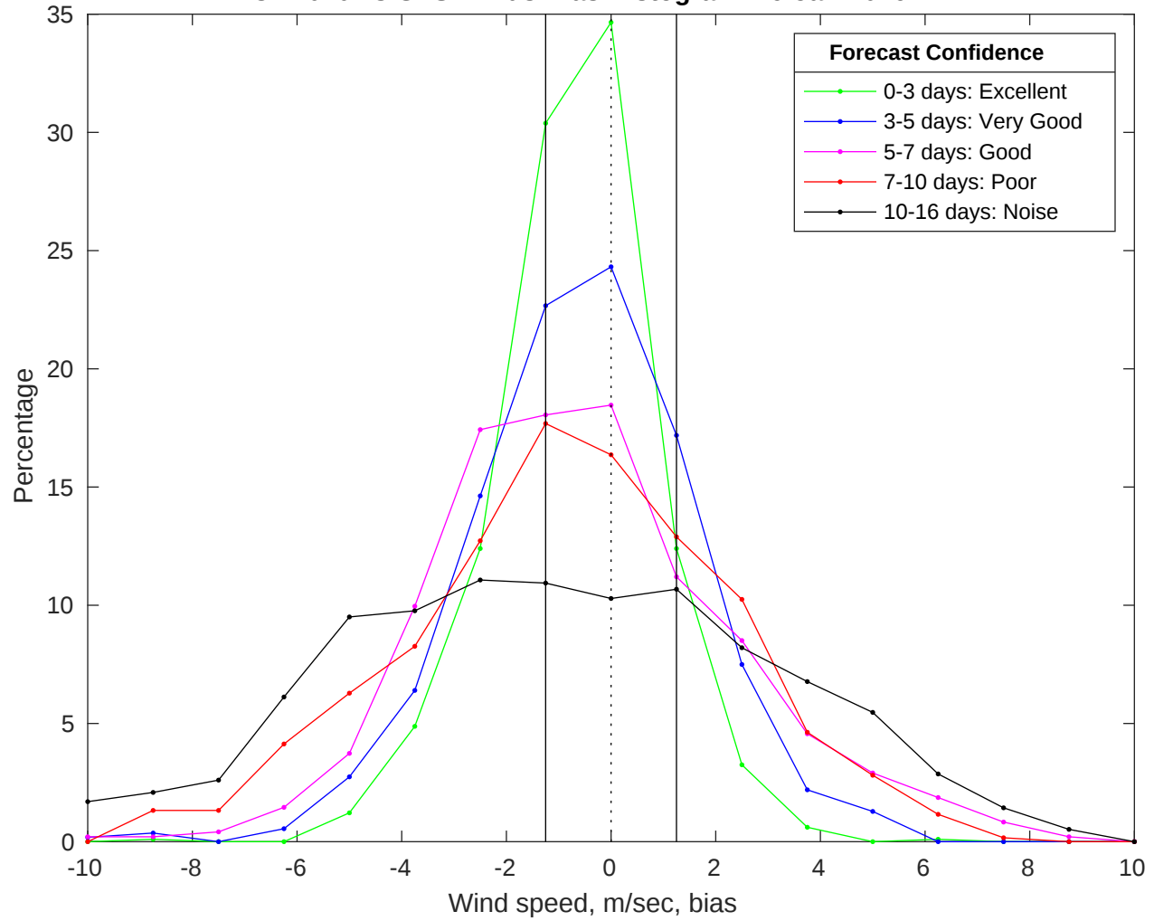
NDBC 42040 vs GFS Winds Bias Histogram: 19-Jan-2026
