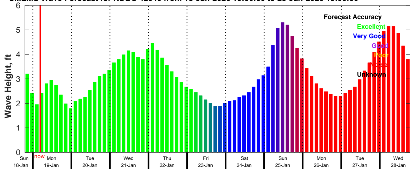
CMEMS Wave Forecast for NDBC 42040 from 18-Jan-2026 19:00:00 to 28-Jan-2026 19:00:00
