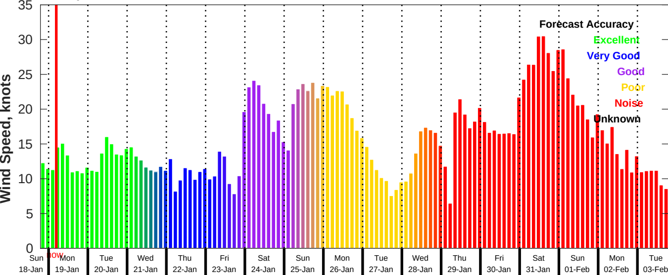
GFS Wind Speed Forecast for NDBC 42040 from 18-Jan-2026 19:00:00 to 03-Feb-2026 19:00:00
