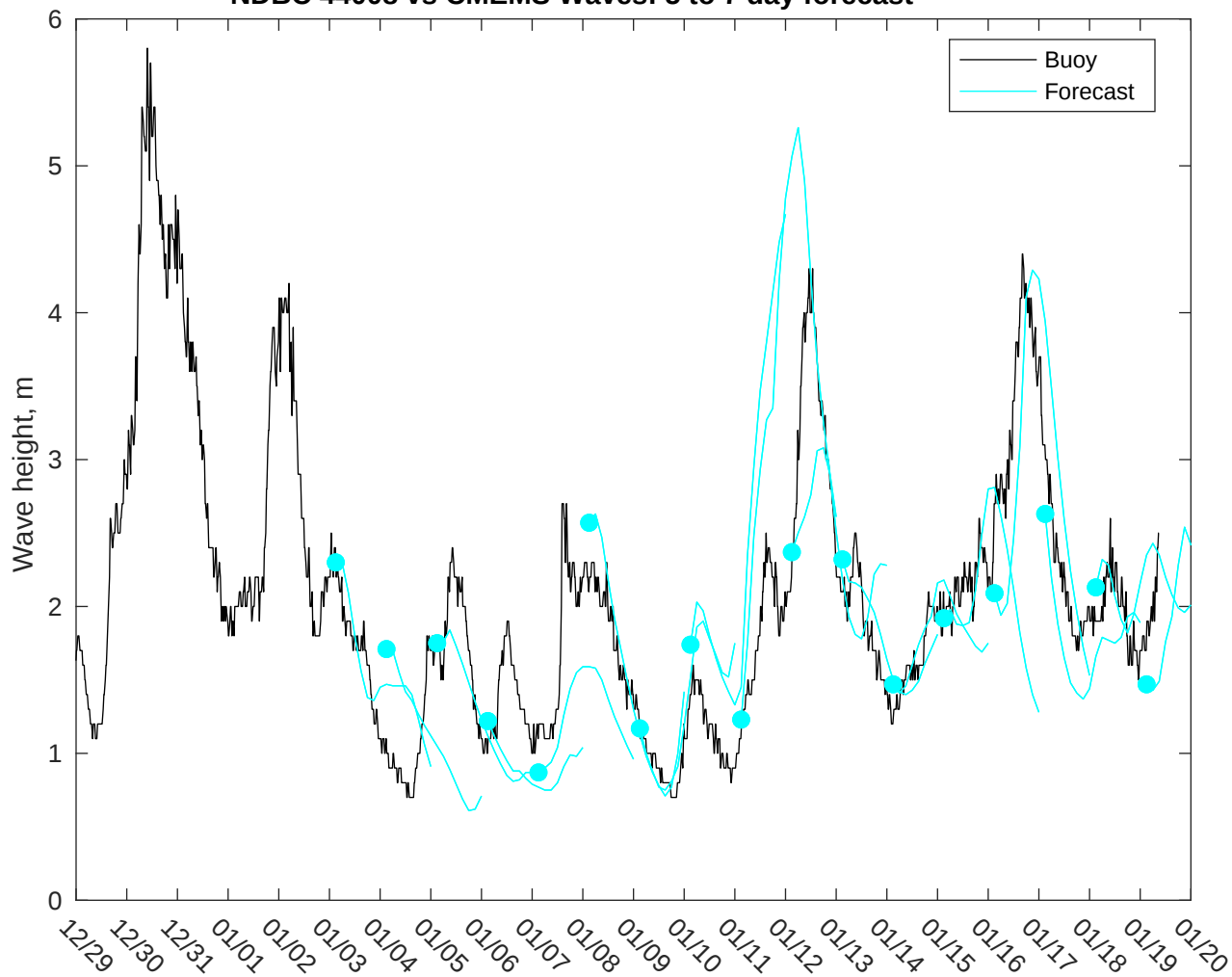
NDBC 44008 vs CMEMS Waves: 5 to 7 day forecast
