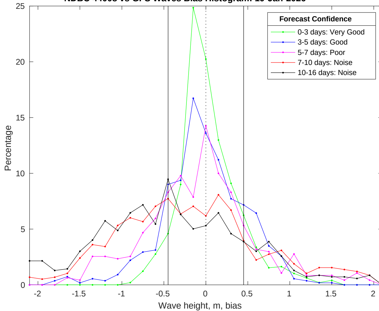
NDBC 44008 vs GFS Waves Bias Histogram: 19-Jan-2026
