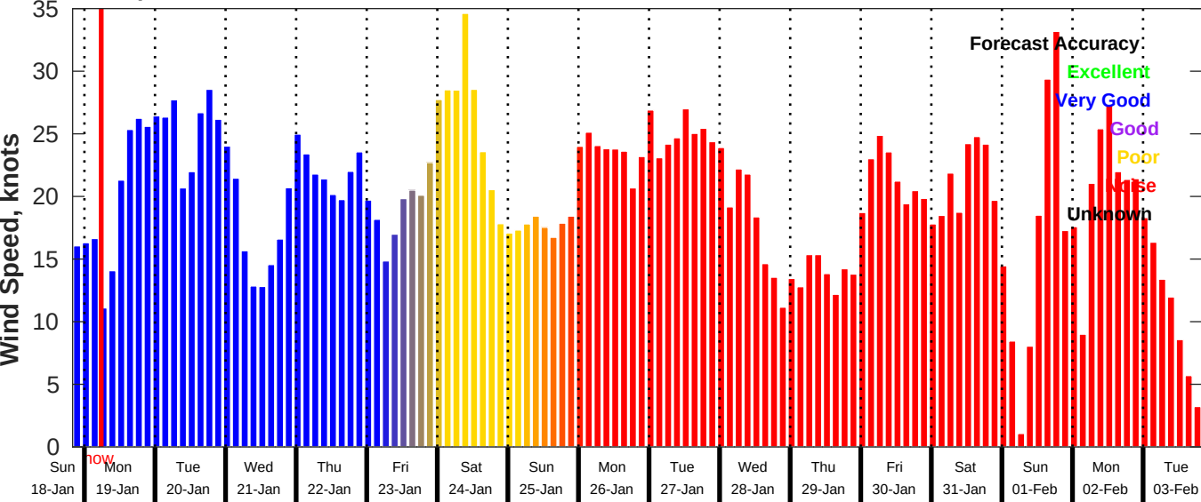
GFS Wind Speed Forecast for NDBC 44008 from 18-Jan-2026 20:00:00 to 03-Feb-2026 20:00:00
