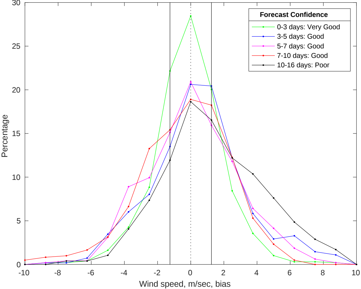
NDBC 46011 vs GFS Winds Bias Histogram: 19-Jan-2026
