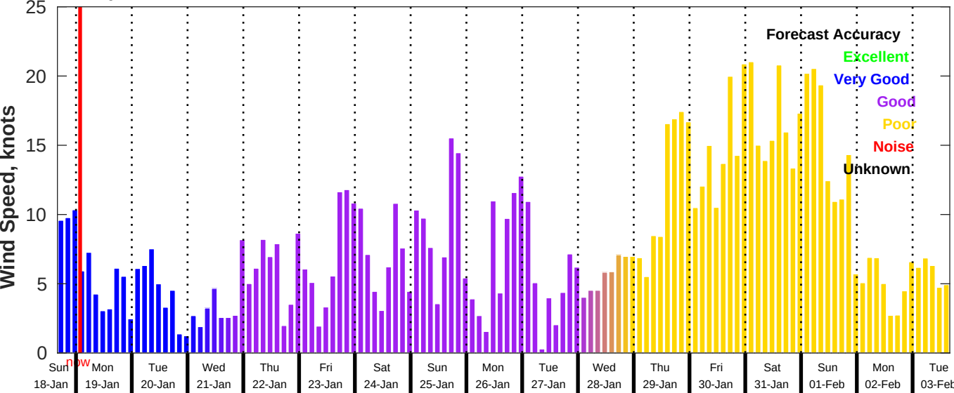
GFS Wind Speed Forecast for NDBC 46011 from 18-Jan-2026 16:00:00 to 03-Feb-2026 16:00:00
