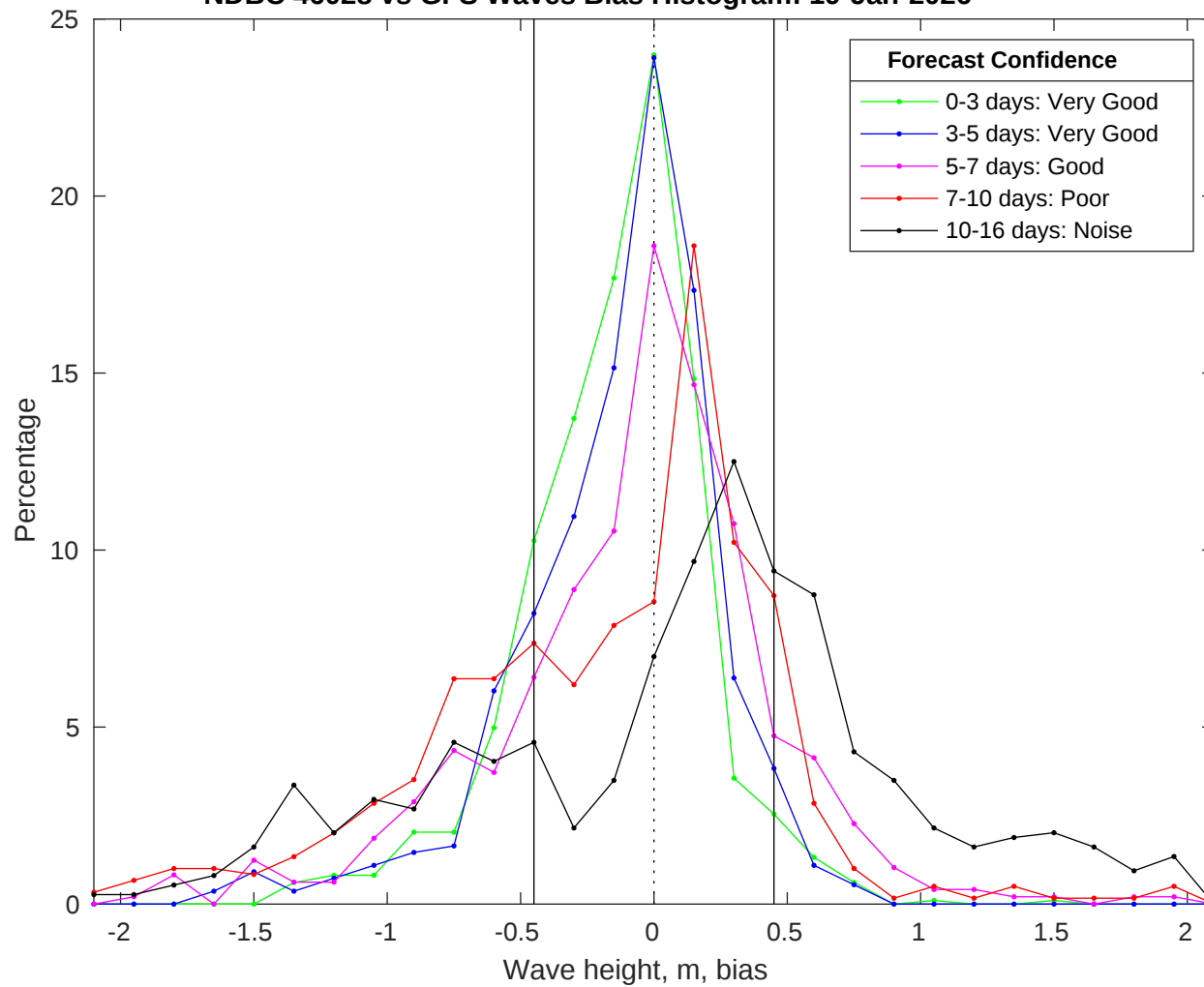
NDBC 46028 vs GFS Waves Bias Histogram: 19-Jan-2026
