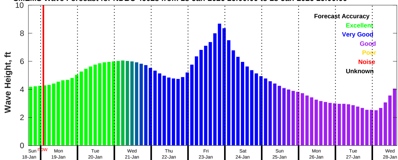
CMEMS Wave Forecast for NDBC 46028 from 18-Jan-2026 16:00:00 to 28-Jan-2026 16:00:00
