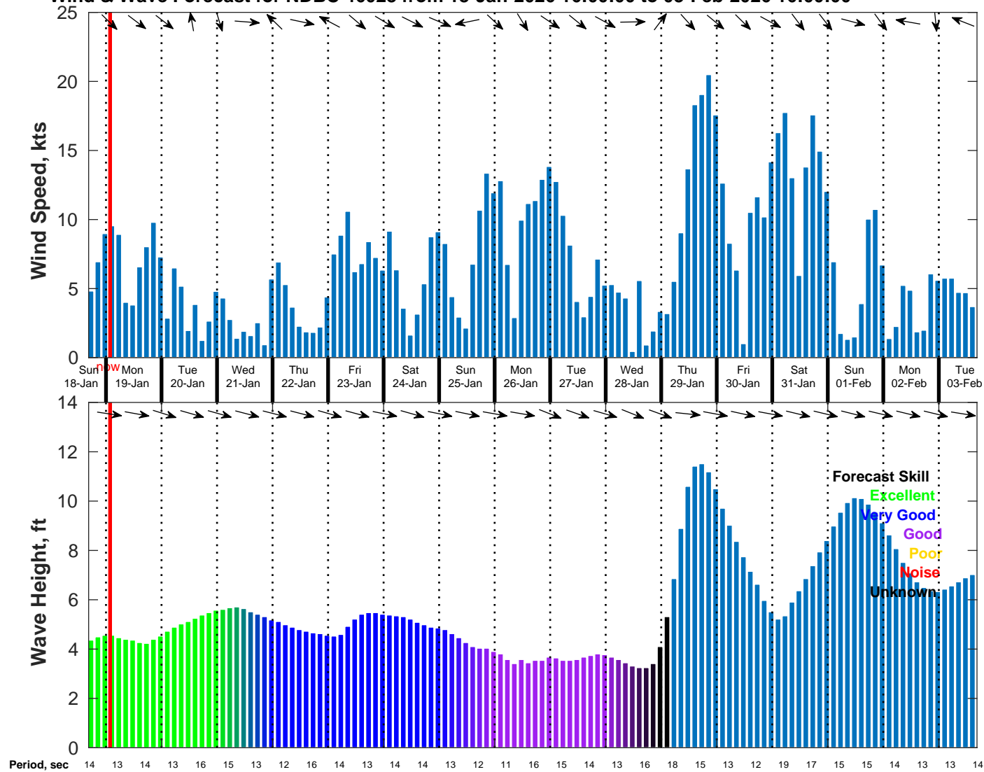
Wind & Wave Forecast for NDBC 46028 from 18-Jan-2026 16:00:00 to 03-Feb-2026 16:00:00
