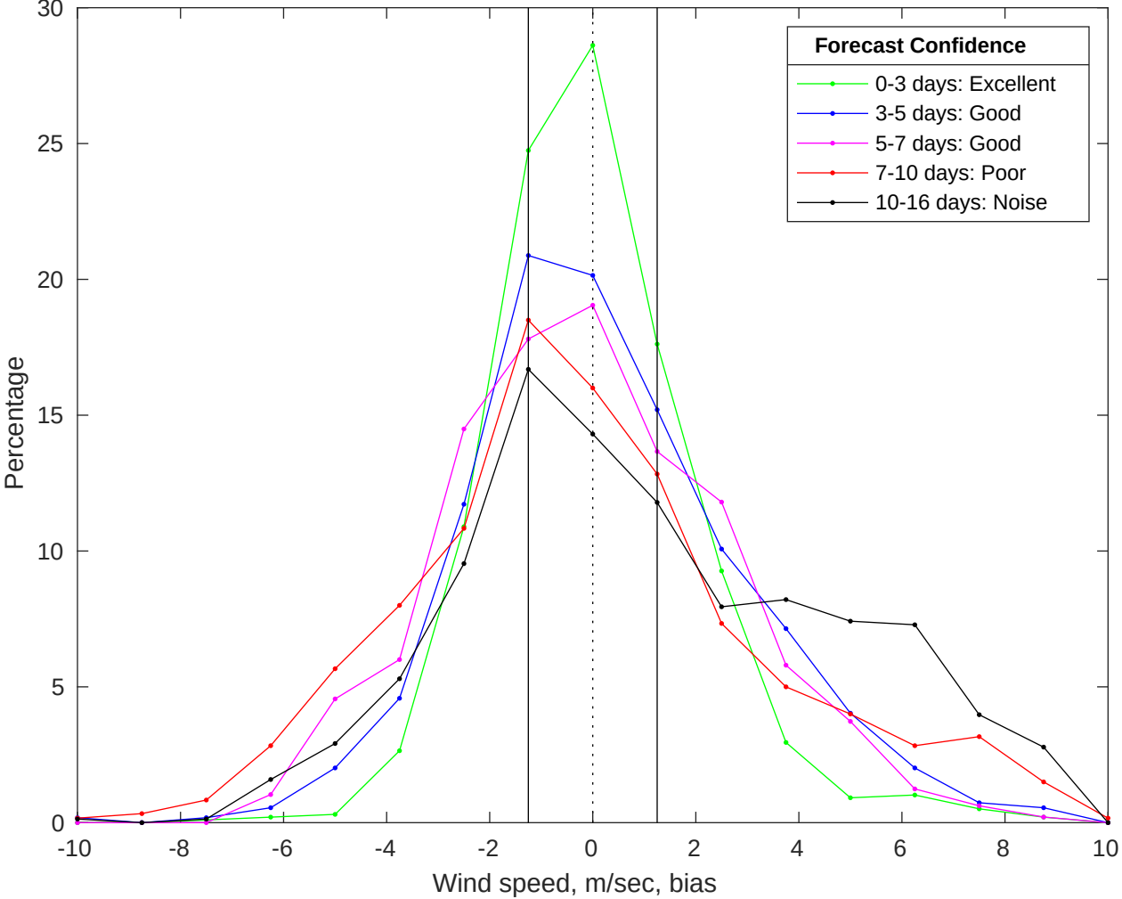
NDBC 46054 vs GFS Winds Bias Histogram: 19-Jan-2026
