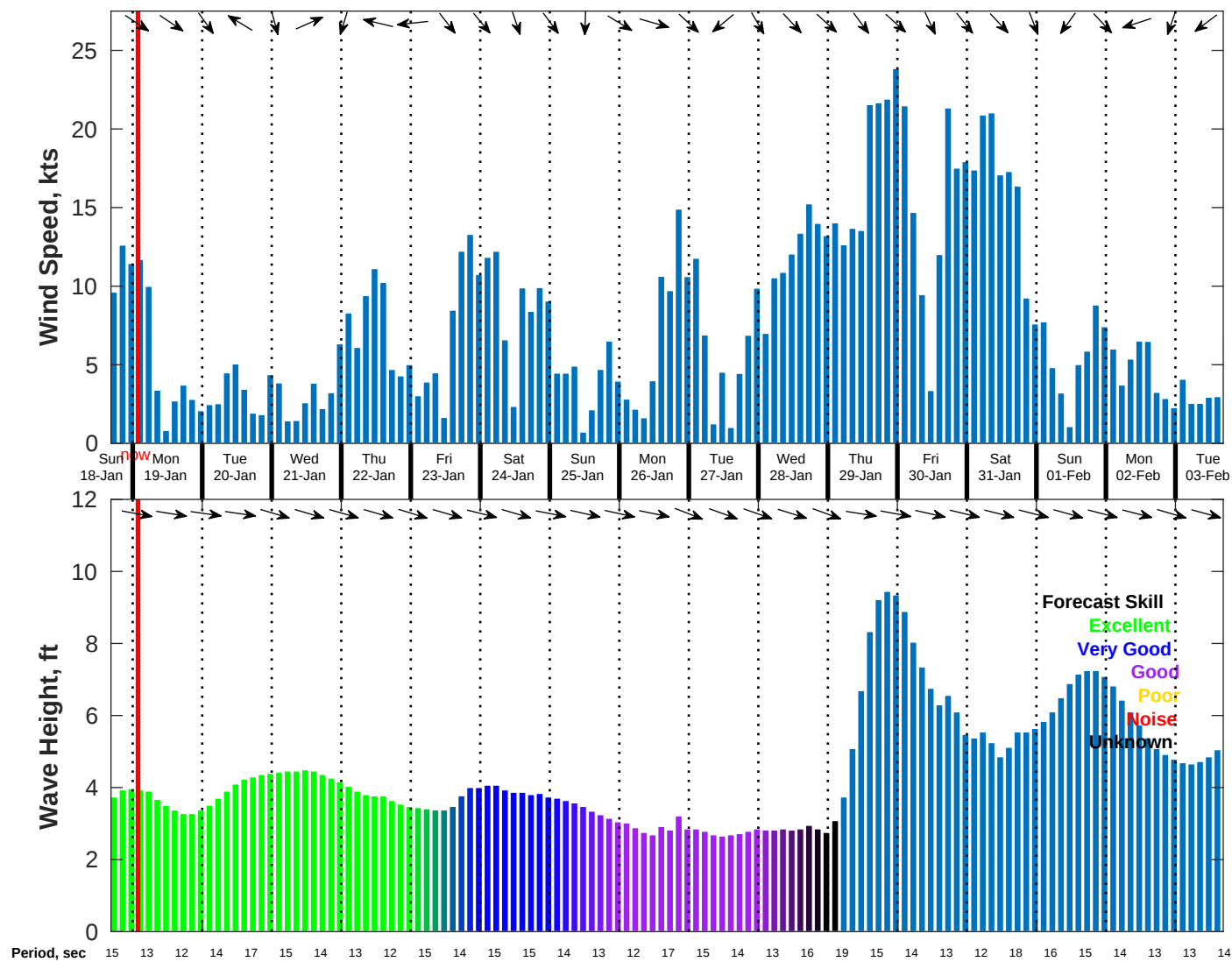
Wind & Wave Forecast for NDBC 46054 from 18-Jan-2026 16:00:00 to 03-Feb-2026 16:00:00
