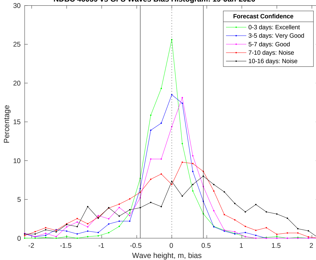
NDBC 46059 vs GFS Waves Bias Histogram: 19-Jan-2026
