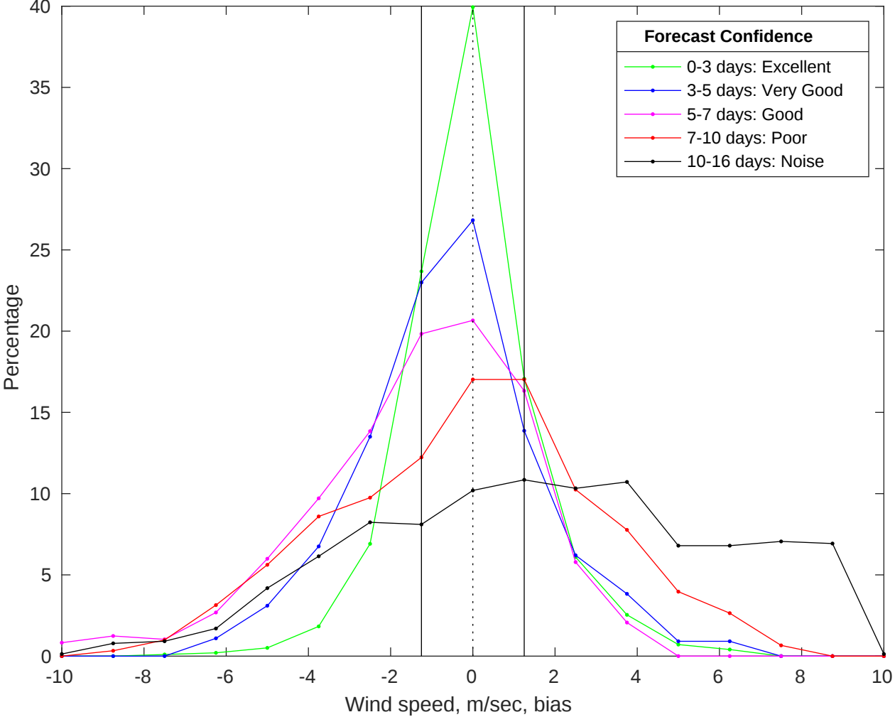
NDBC 46059 vs GFS Winds Bias Histogram: 19-Jan-2026
