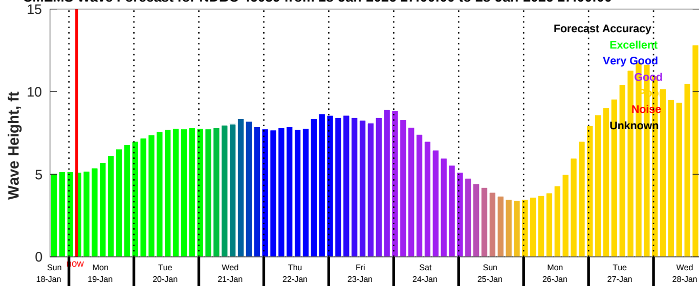
CMEMS Wave Forecast for NDBC 46059 from 18-Jan-2026 17:00:00 to 28-Jan-2026 17:00:00
