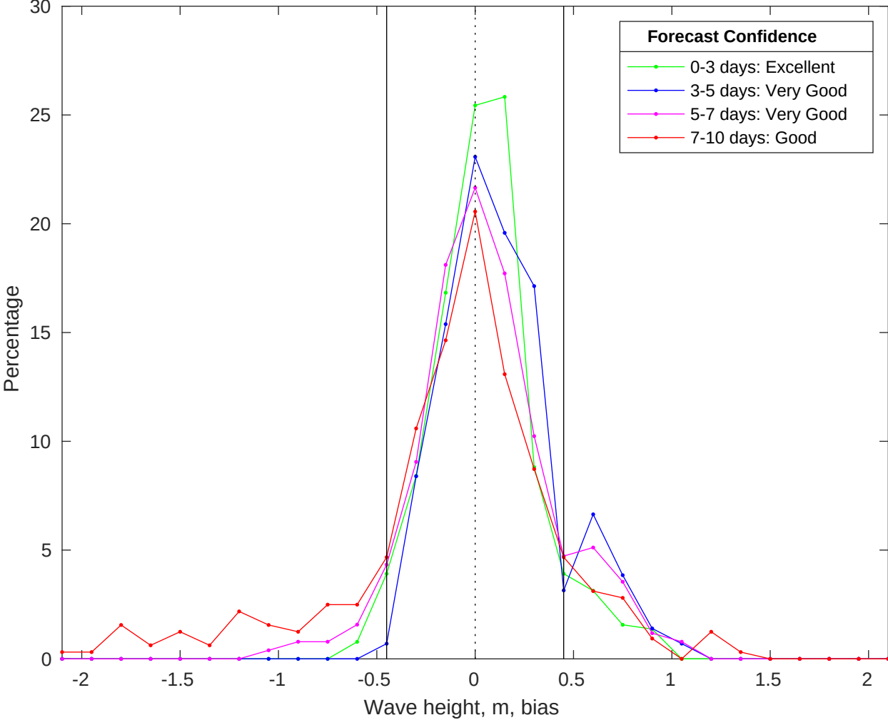
NDBC 46069 vs CMEMS Waves Bias Histogram: 19-Jan-2026
