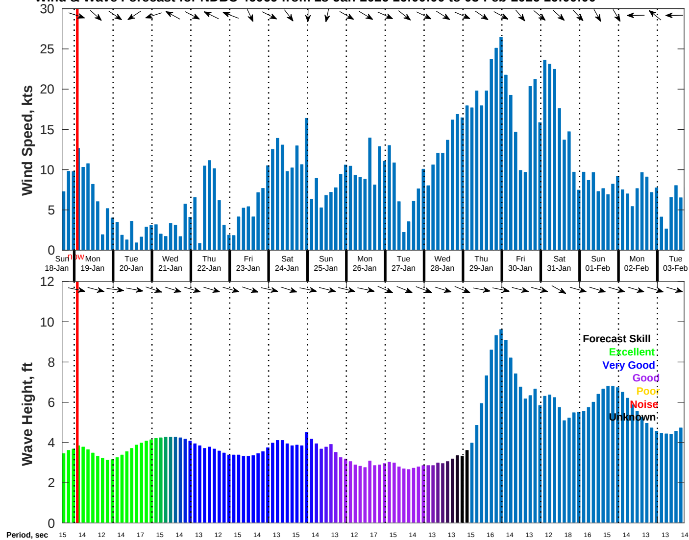
Wind & Wave Forecast for NDBC 46069 from 18-Jan-2026 16:00:00 to 03-Feb-2026 16:00:00
