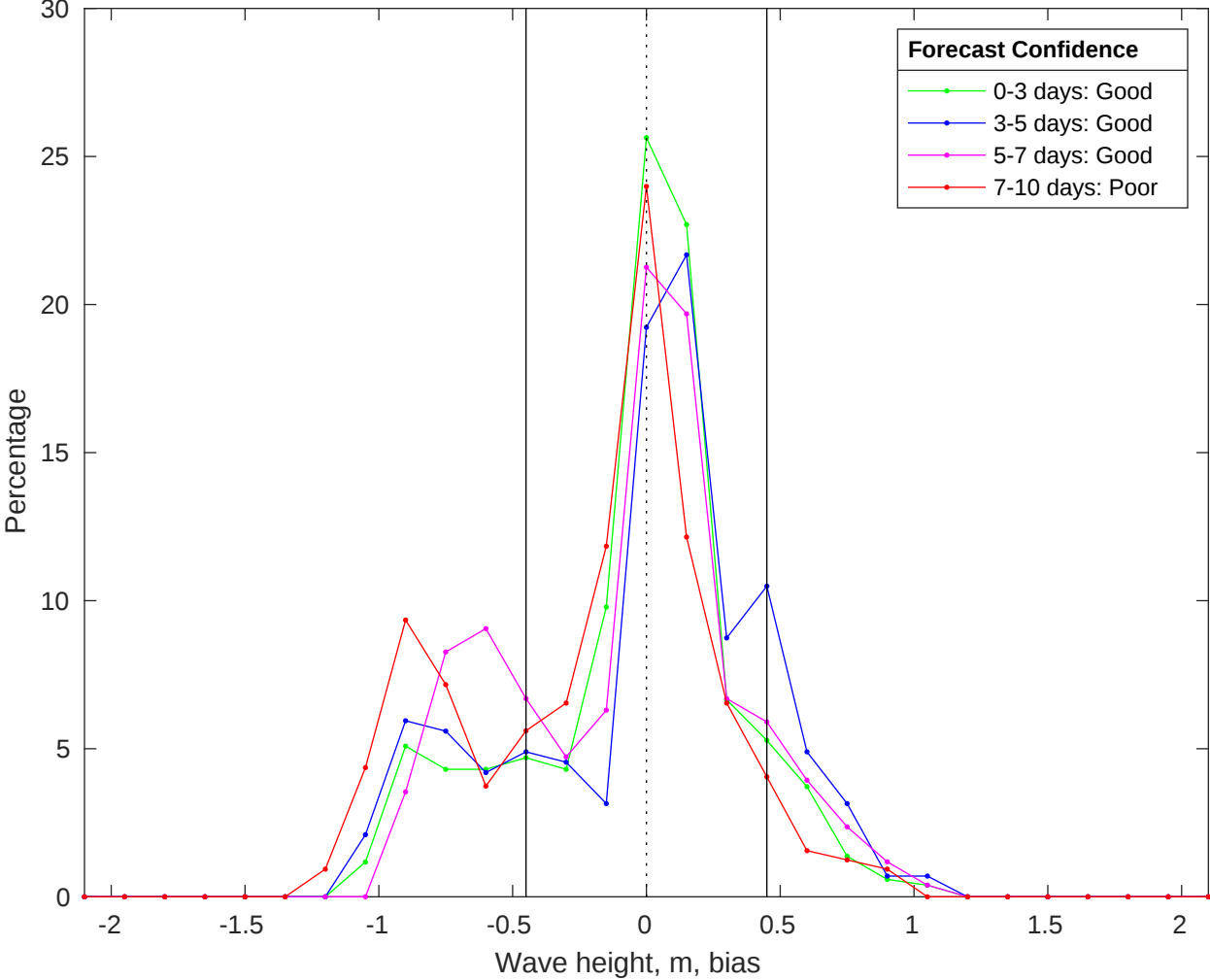
NDBC 46215 vs CMEMS Waves Bias Histogram: 19-Jan-2026
