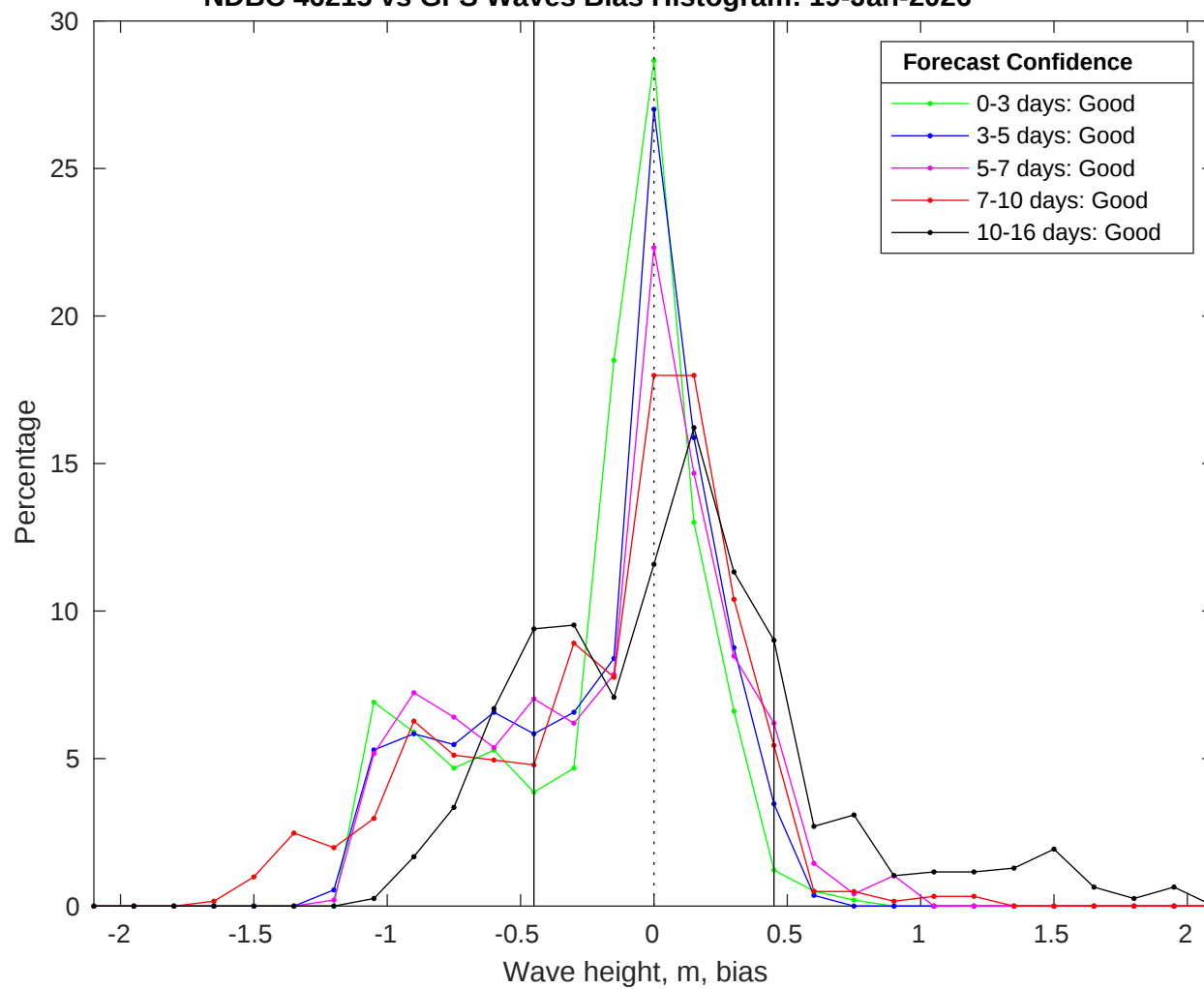
NDBC 46215 vs GFS Waves Bias Histogram: 19-Jan-2026
