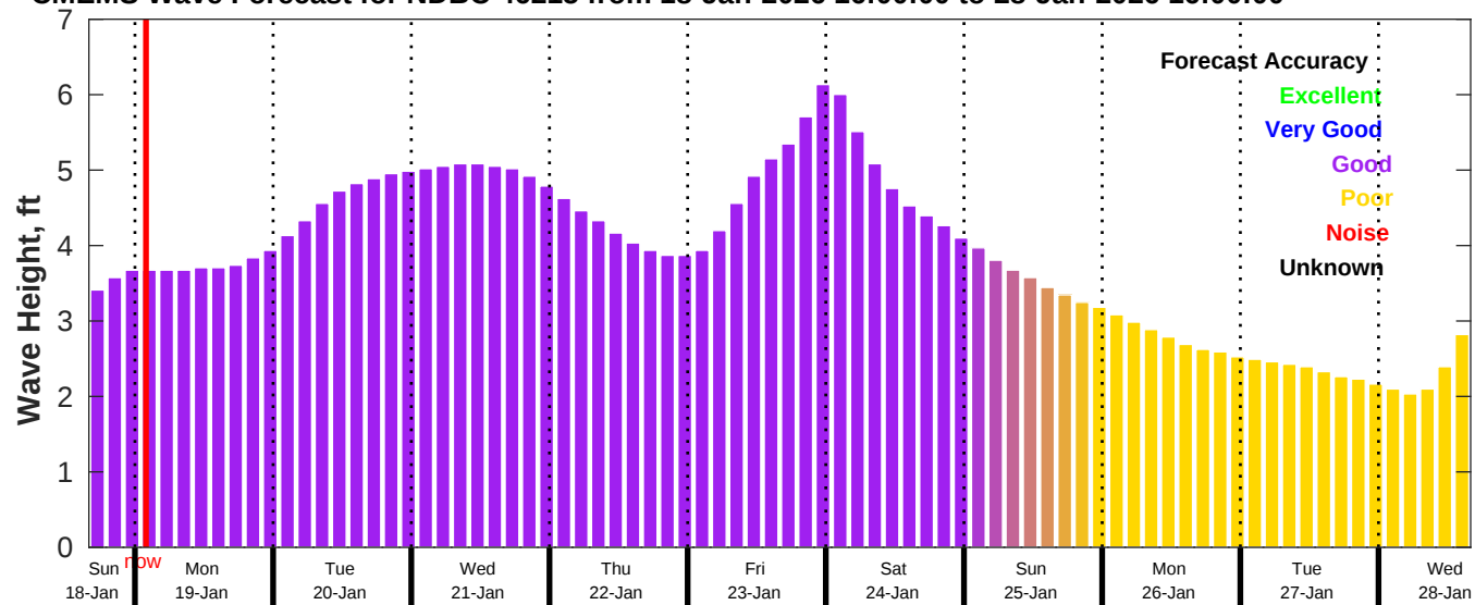
CMEMS Wave Forecast for NDBC 46215 from 18-Jan-2026 16:00:00 to 28-Jan-2026 16:00:00
