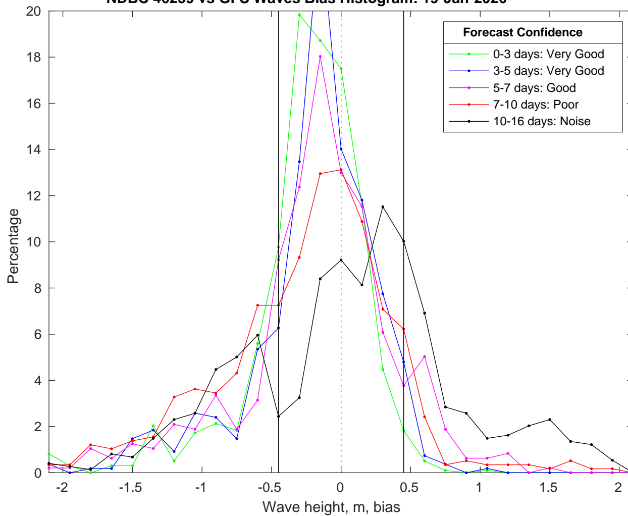
NDBC 46259 vs GFS Waves Bias Histogram: 19-Jan-2026
