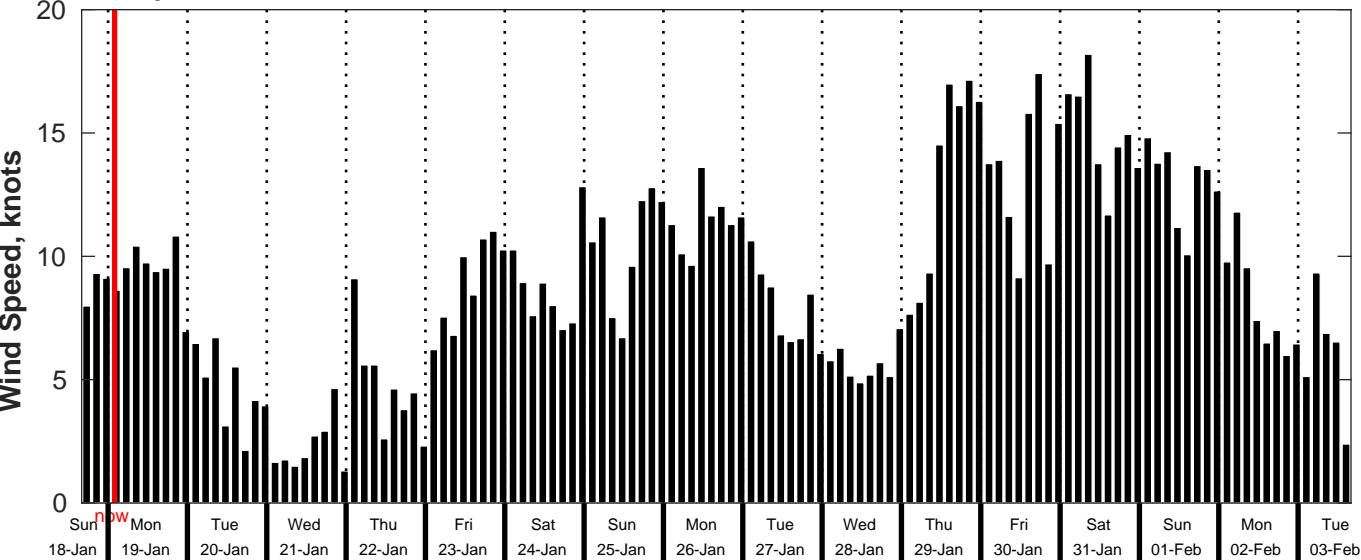
GFS Wind Speed Forecast for NDBC 46259 from 18-Jan-2026 16:00:00 to 03-Feb-2026 16:00:00
