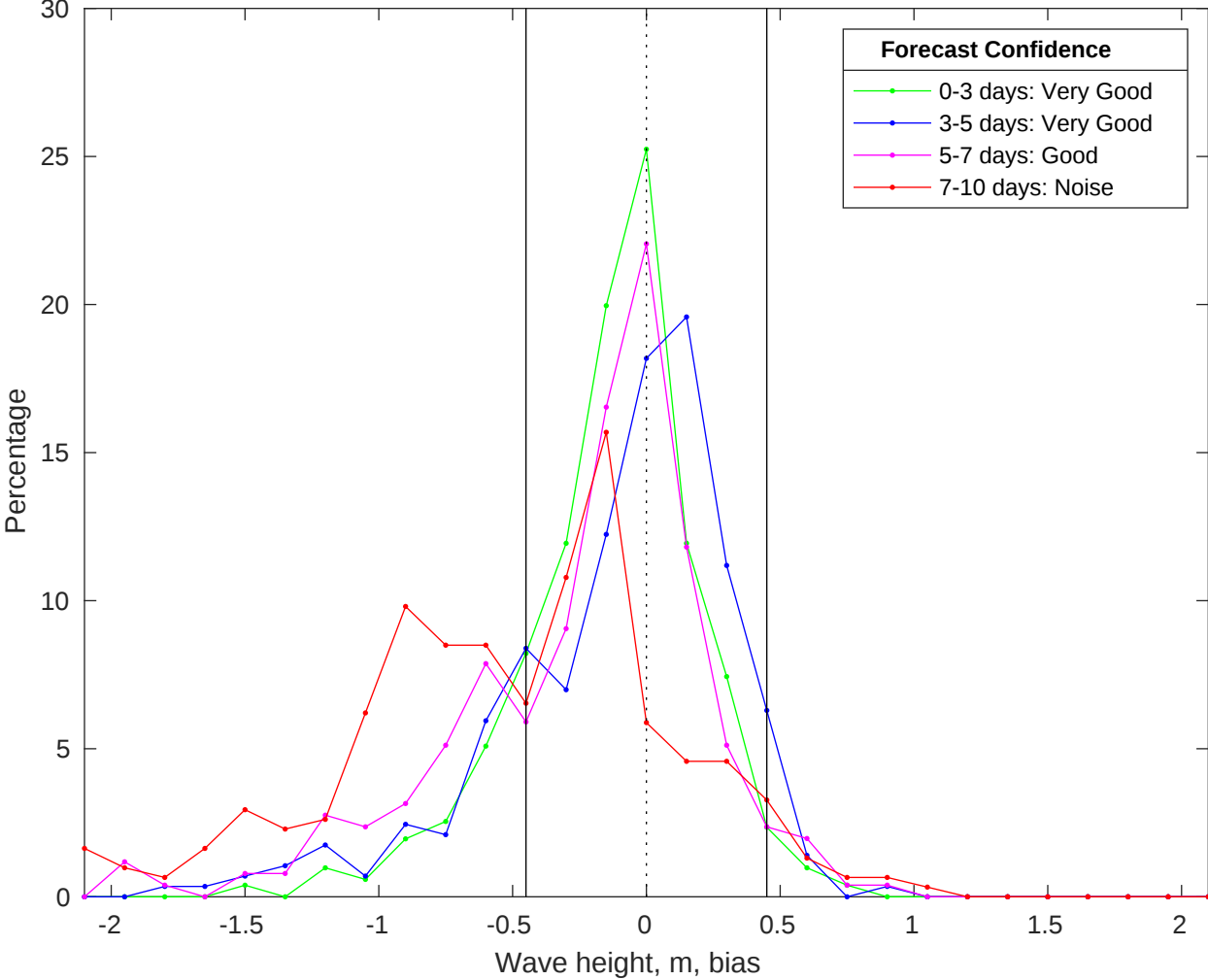
NDBC 51000 vs CMEMS Waves Bias Histogram: 19-Jan-2026
