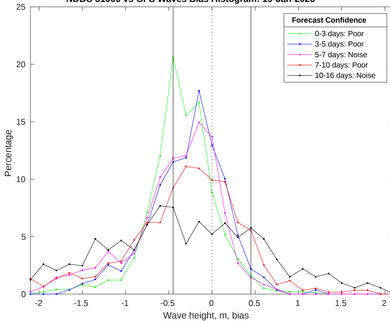
NDBC 51000 vs GFS Waves Bias Histogram: 19-Jan-2026
