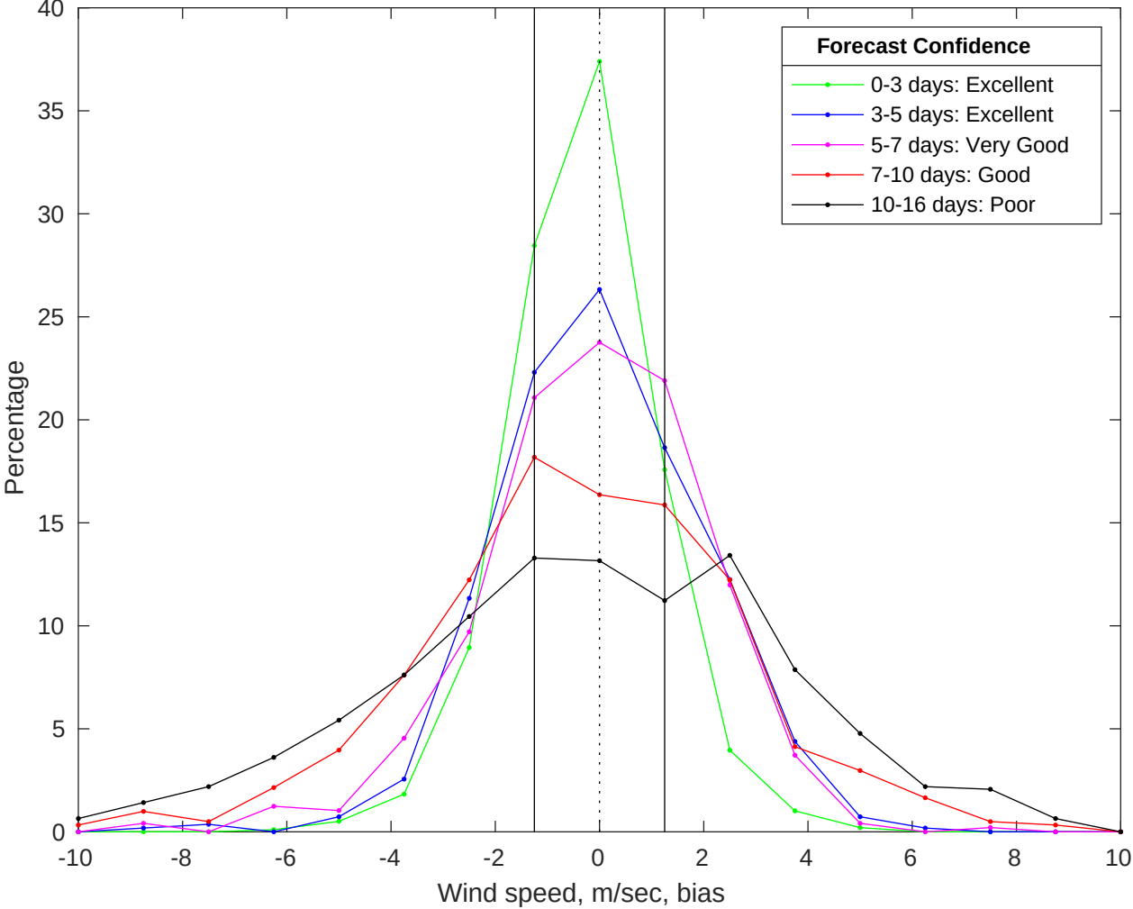
NDBC 51000 vs GFS Winds Bias Histogram: 19-Jan-2026
