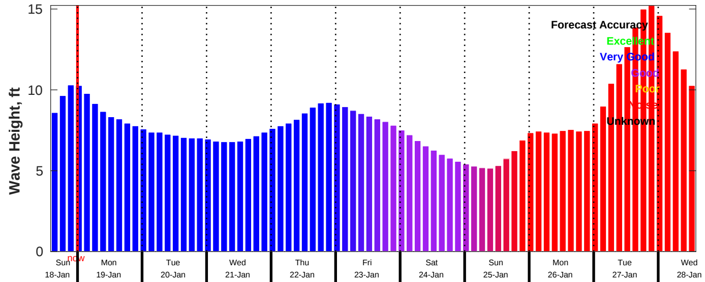
CMEMS Wave Forecast for NDBC 51000 from 18-Jan-2026 14:00:00 to 28-Jan-2026 14:00:00
