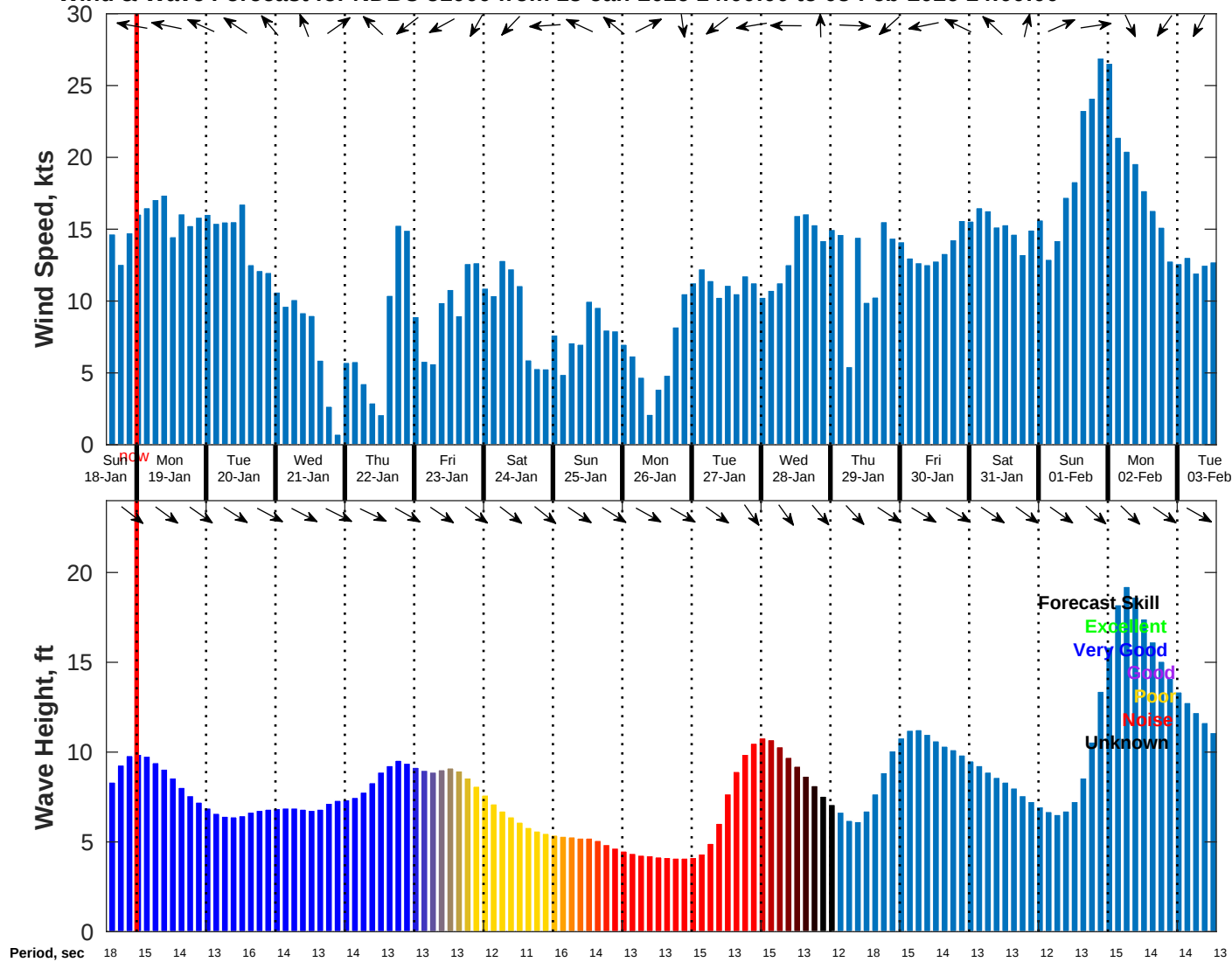
Wind & Wave Forecast for NDBC 51000 from 18-Jan-2026 14:00:00 to 03-Feb-2026 14:00:00
