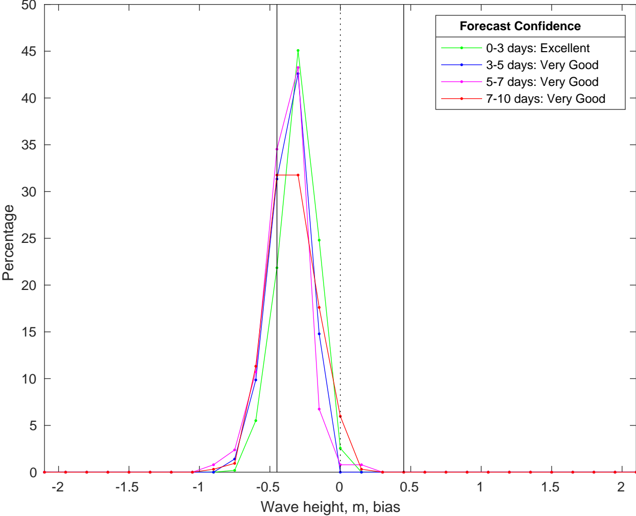
NDBC 51209 vs CMEMS Waves Bias Histogram: 19-Jan-2026
