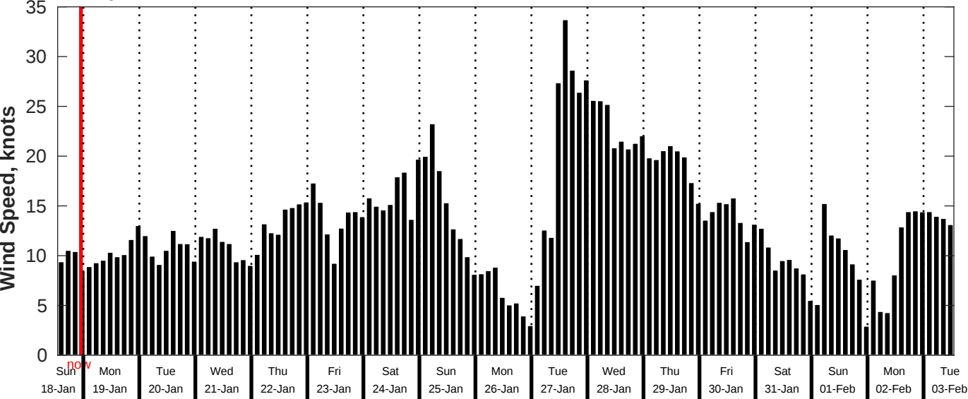
GFS Wind Speed Forecast for NDBC 51209 from 18-Jan-2026 13:00:00 to 03-Feb-2026 13:00:00
