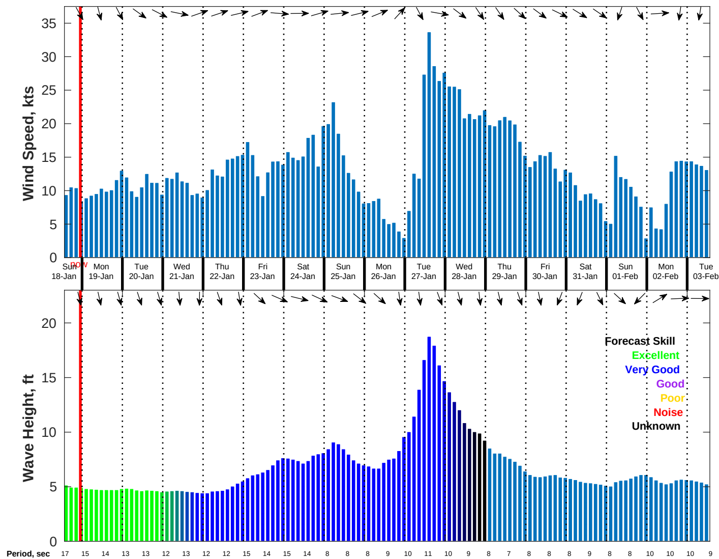
Wind & Wave Forecast for NDBC 51209 from 18-Jan-2026 13:00:00 to 03-Feb-2026 13:00:00
