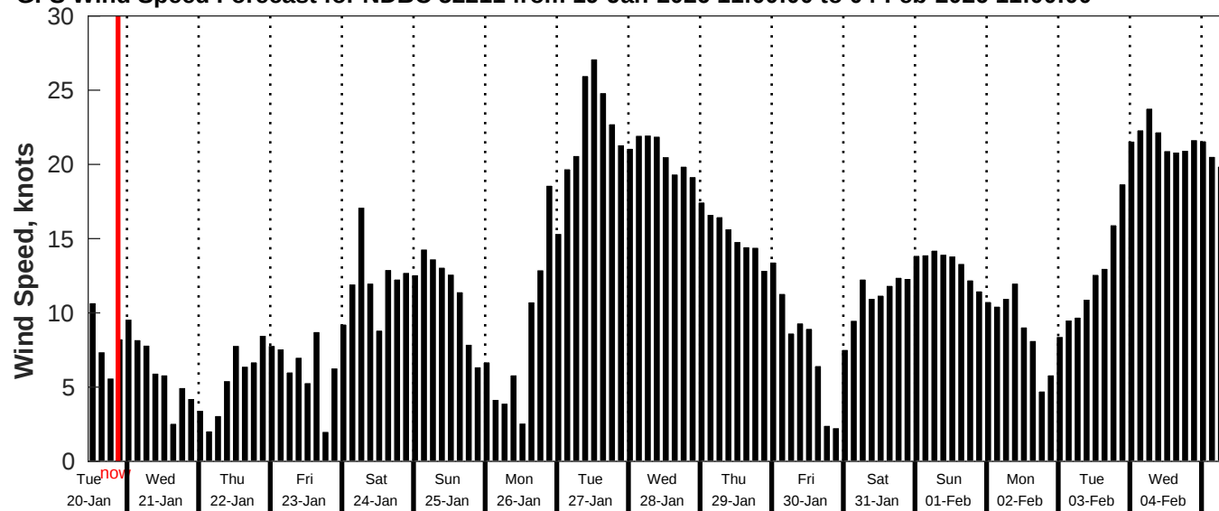
GFS Wind Speed Forecast for NDBC 52211 from 19-Jan-2026 11:00:00 to 04-Feb-2026 11:00:00
