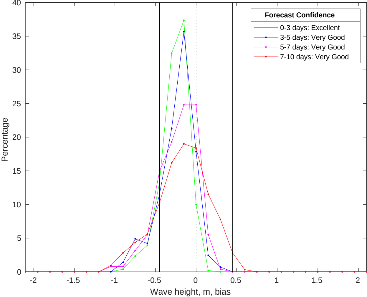
NDBC 52213 vs CMEMS Waves Bias Histogram: 19-Jan-2026
