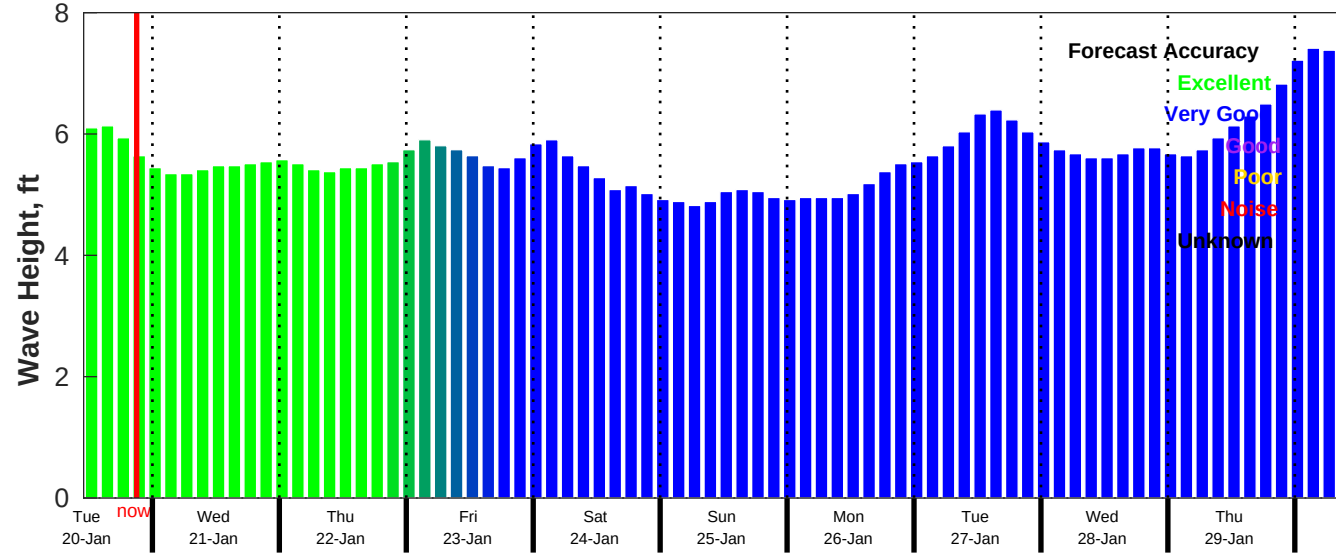
CMEMS Wave Forecast for NDBC 52213 from 19-Jan-2026 11:00:00 to 29-Jan-2026 11:00:00
