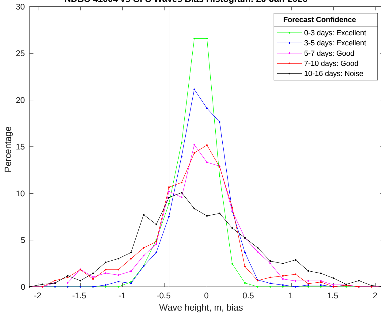
NDBC 41004 vs GFS Waves Bias Histogram: 20-Jan-2026
